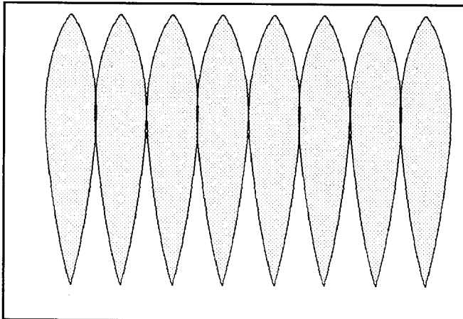
Figure 4: If our envelope were unrolled, evenly sized pieces of fabric, commonly called 'gores' would appear.
