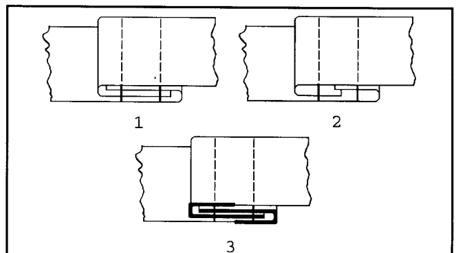
Figure 5: Drawings 1 and 2 show variations in the French Fell or folded fell seam, commonly used for envelope construction. The highlighted lines in drawing 3 represent the fabric contained within the seam allowance .
